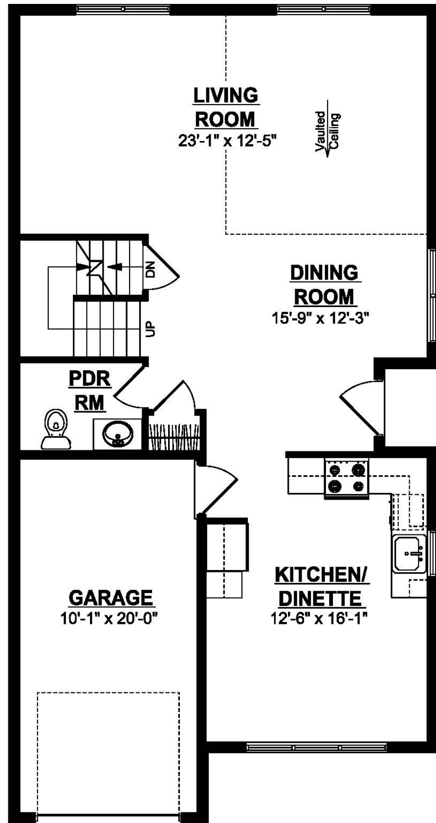
FIRST FLOOR PLAN UNIT B
