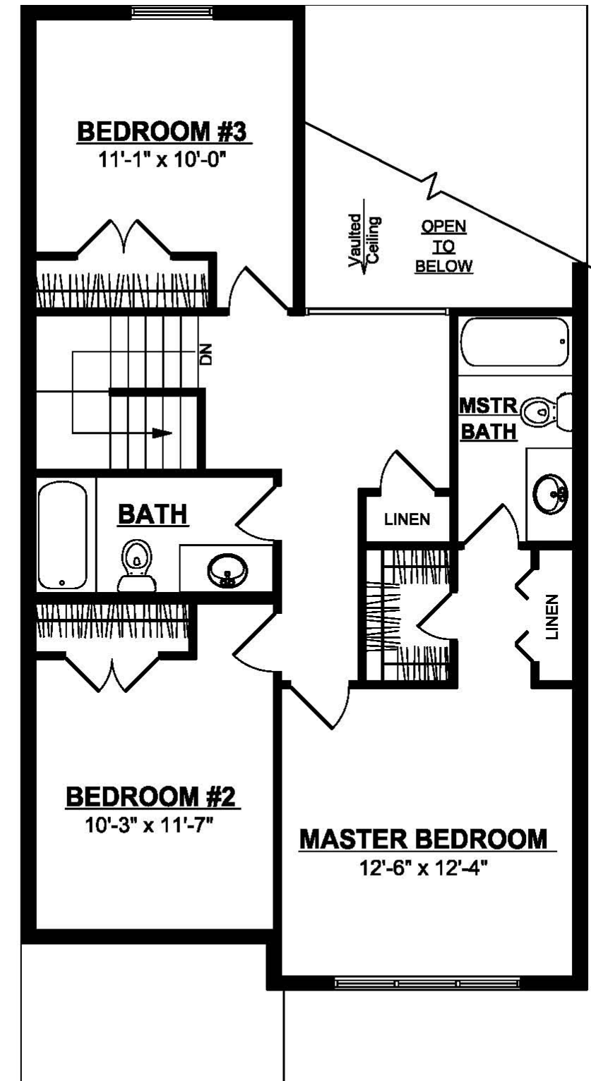
SECOND FLOOR PLAN UNIT B
